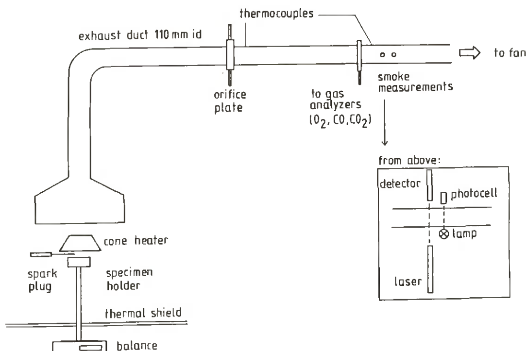
Figure 1. Cone Calorimeter.
